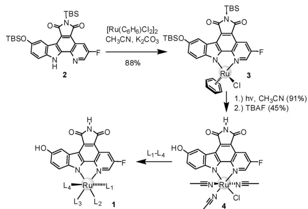
Figure 3. Synthesis of octahedral Ru complexes 1 from precursor 4 .
