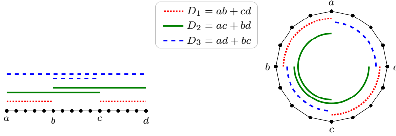
Fig. 1 Two illustrative examples for the four-point condition. Left : A path P_{16} with 16 vertices; Right : A cycle C_{16} with 16 vertices. Indeed, \delta(P_{16}) = 0 , here indicated by the equally largest two distance sums D_2 (solid) and D_3 (dashed). The situation changes in the case of a C_{16} (that is, the P_{16} with one additional edge connecting the endpoints). We have \delta(C_{16}) = 8 , here indicated by the largest distance sum D_2 (solid) and the two equally smallest distance sums D_1 (dotted) and D_3 (dashed).
