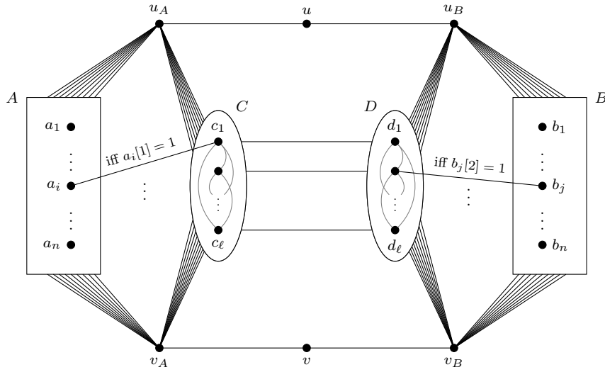
Fig. 3 Sketch of the construction described in the proof of Theorem 5 . Ellipses indicate cliques, rectangles indicate independent sets. Multiple edges to an object indicate that the corresponding vertex is incident to each vertex enclosed within that object.
