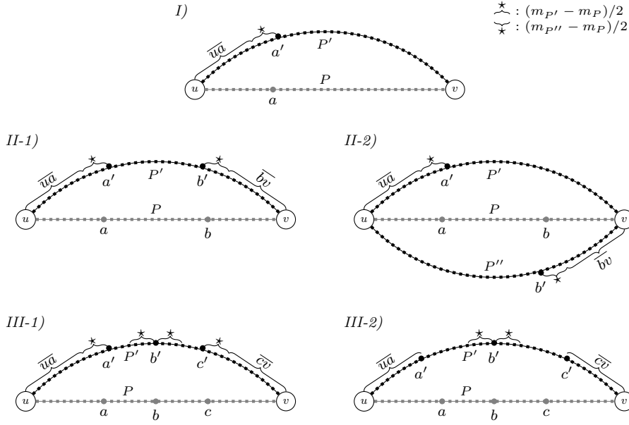
Fig. 2 Illustrations to the cases I-III and the subcases therein in the proof of Lemma 7 .
