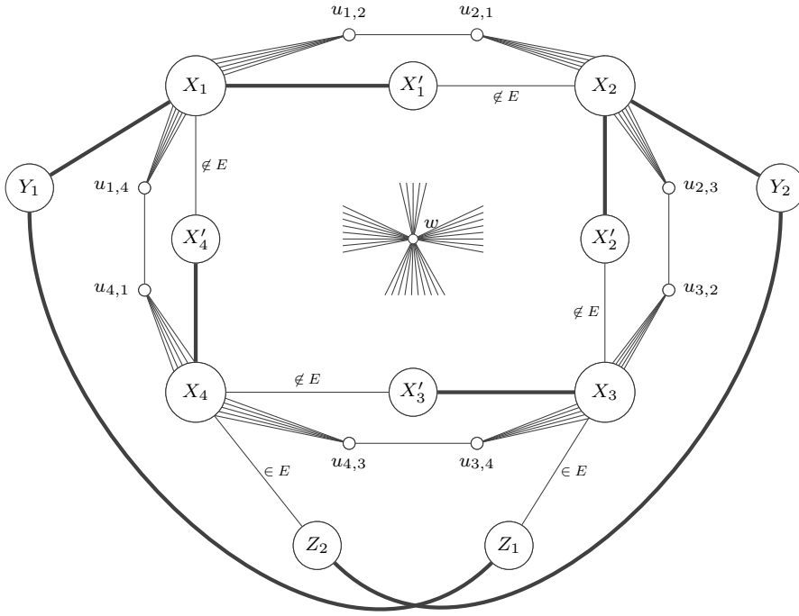
Fig. 4 An illustrative sketch of the graph constructed in the proof of Theorem 8 . Encircled vertices correspond to cliques. A thick edge represents a matching between copy-vertices. An edge labeled “ \in E ” (“ \notin E ”) represent incidences corresponding to present (not present) edges in the original graph. The vertex w is incident with all vertices except vertices contained in X_i for all 1 \leq i \leq 4 .
