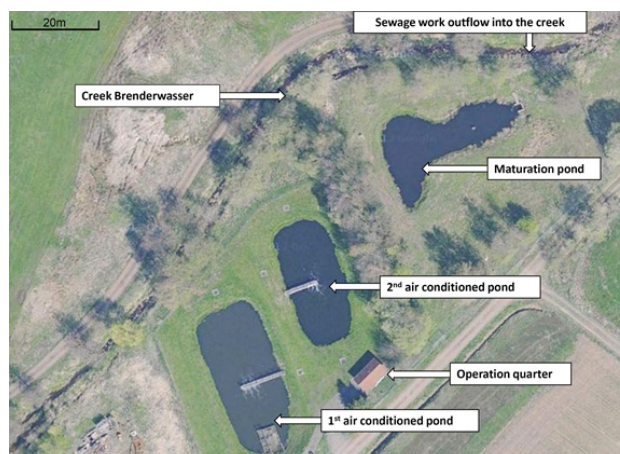
Photo 3 Pond sewage plant in Dirlammen. Source: Own elaboration, based on Google Maps 2013
