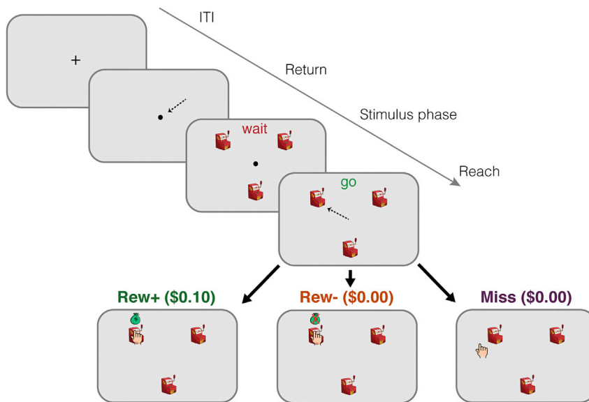
Figure 1. Task Design
