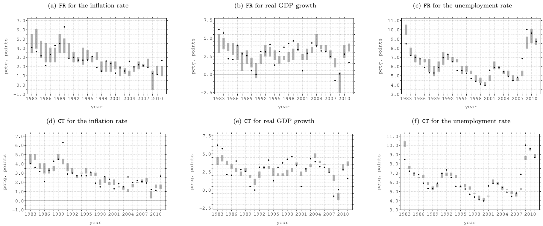
Fig. A.2: 12-month-ahead interval projections and realizations
