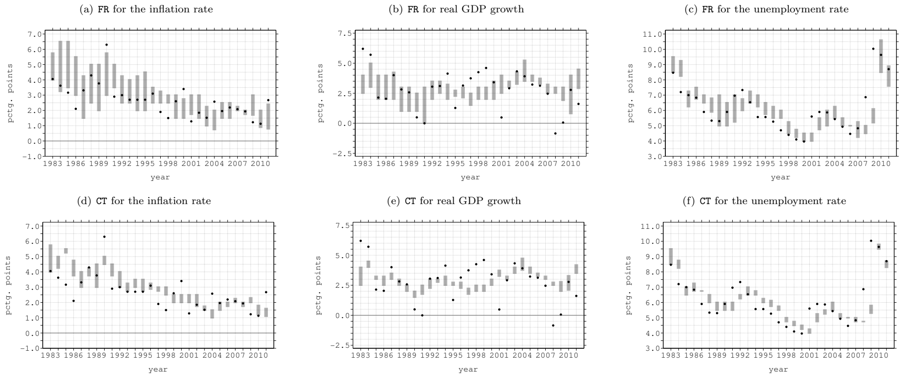
Fig. A.3: 18-month-ahead interval projections and realizations
