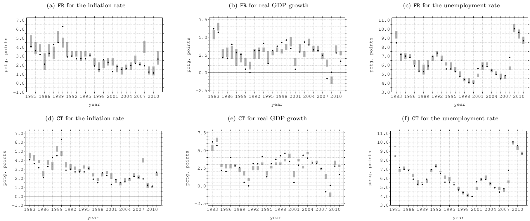
Fig. A.1: 6-month-ahead interval projections and realizations
