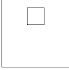
FIGURE 3. \text{supp } \psi_\lambda \not\subset \overline{\Xi_{\lambda', i'}} for any 1 \leq i' \leq m , i.e., an entry of \mathbf{M}^{(s)} , but \Xi_{\lambda, i} \subset \Xi_{\lambda', i'(i)} for any i .
