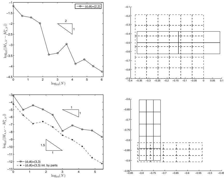
FIGURE 10. Quadrature errors for single entries of \mathbf{M}^{(s)} for different granularities N with p = d = \tilde{d} = 2 (top left) and p = 4, d = \tilde{d} = 3 (bottom left), respectively. The right pictures show the singular supports of the wavelets involved. The dotted line in the lower left picture refers to the case where the composite rule was applied to the right hand side of (3.8).
