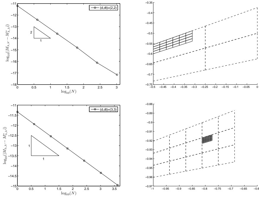
FIGURE 7. Quadrature errors for single entries of \mathbf{M}^{(r)} for different granularities N and p = 4 (and d = \tilde{d} = 2 ) and p = 2 ( d = \tilde{d} = 3 ), respectively. The right pictures show the the singular supports of the wavelets involved.
