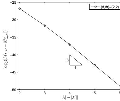
FIGURE 8. Decay of the quadrature error in a column of \mathbf{M}^{(r)} as function of ||\lambda| - |\lambda'|| for fixed N , and p = d = \tilde{d} = 2 .
