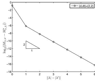
FIGURE 9. Decay of the quadrature error for entries \mathbf{M}_{\lambda, \lambda'}^{(s)} as function of \|\lambda\| - \|\lambda'\| for fixed \lambda' and N , p = d = \tilde{d} = 2 , where the singular supports of \psi_\lambda and \psi_{\lambda'} are nested like in Figure 3, because \lambda = (i, \mu) and \lambda' = (i, \mu') , i.e., they are lifted by the same \kappa_i .
