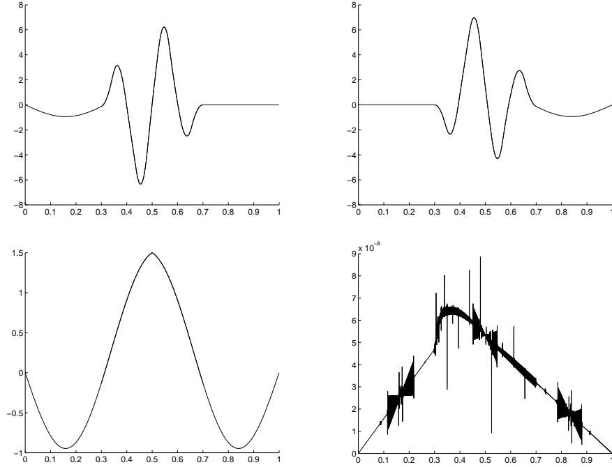
FIGURE 5. Final local approximations u_{2k}^{(0)} (upper left), u_{2k}^{(1)} (upper right), produced by MultSchw and the corresponding global approximation u_{2k} and global pointwise error for d = 3 , j_0 = 3 .
