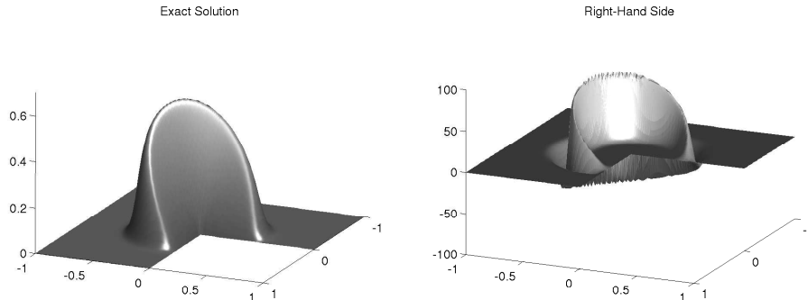
FIGURE 8. Exact solution (left) and right-hand side of the two dimensional test problem.
