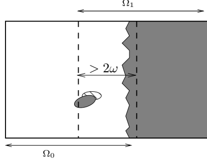
FIGURE 1. \text{supp } \psi_\lambda^{(0)} and \text{supp } \tilde{\psi}_\lambda^{(0)} for \lambda \in \nabla^{(0)} with \text{supp } \psi_\lambda^{(0)} \not\subset \Omega^{(1)} , and \text{supp } u_k^{(1)} for some odd k assuming (3.5).
