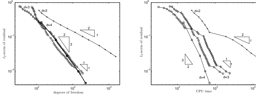
FIGURE 9. \ell_2 -norms of the residuals of \mathbf{u}_k after the application of COARSE versus \#\text{supp } \mathbf{u}_k (left) and versus CPU time (right). Crosses: d = 2 , circles: d = 3 , j_0 = 4 , diamonds: d = 3 , j_0 = 3 , boxes: d = 4 .
