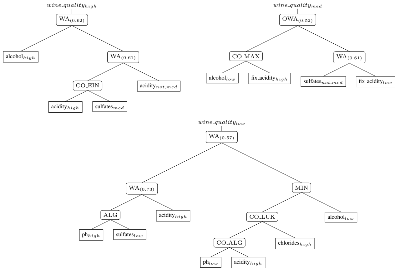
Fig. 5. Pattern trees for the red wine quality data (PT-sys).
