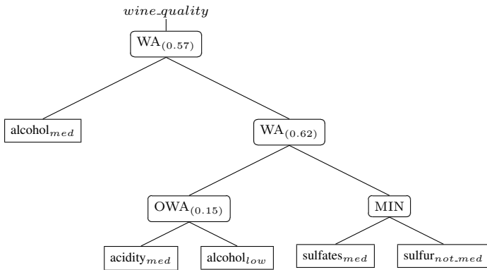
Fig. 4. Pattern tree for red wine quality data (PT-reg).
