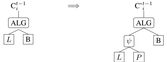
Fig. 3. Top-down induction: A leaf node is expanded through replacement by a basic tree.
