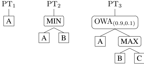
Fig. 1. Examples of simple pattern trees.
